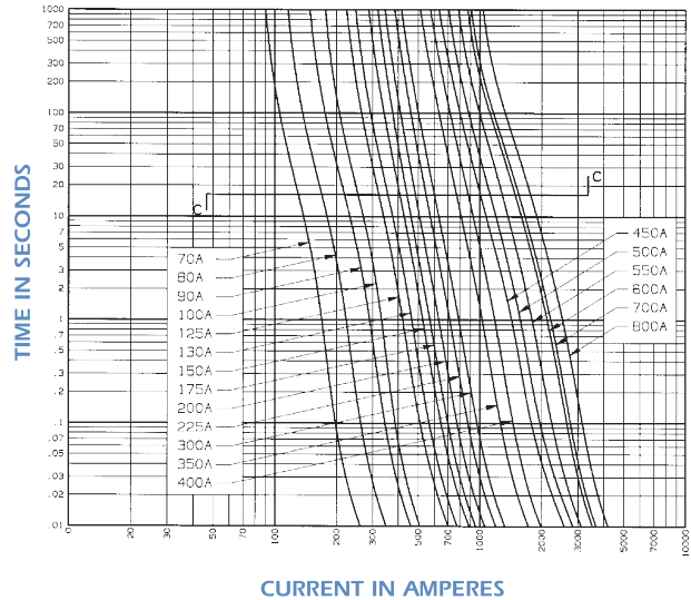
Melting Time - Current Data A30QS 70 to 800
